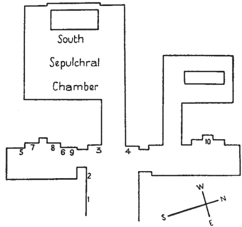
EL-HAGÂRSA. Kaemnefert. From PETRIE, Athribis , pl. v.
